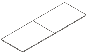
2-Piece Surface Width: 96"-144" Depth: 24"-61" Thickness: 1.25"
