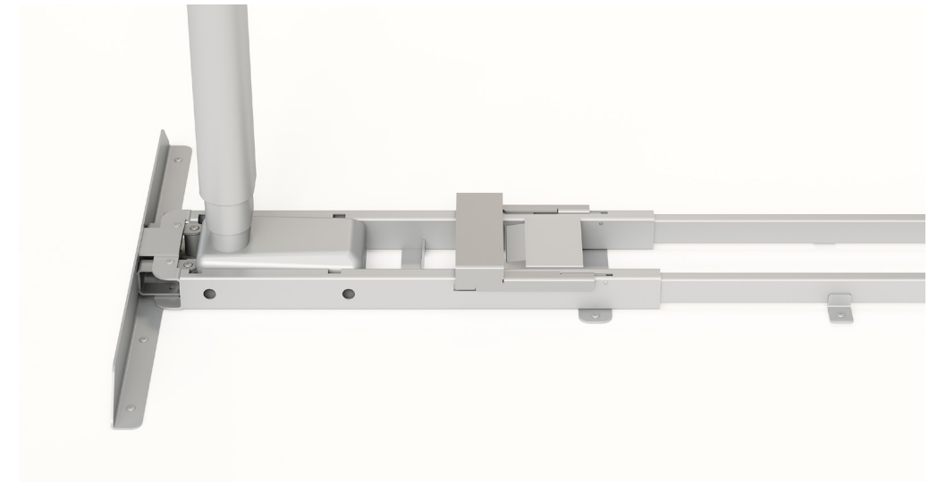
SIMPLY INSERT THE LEG AND EXTEND THE CANTILEVERS TO LOCK INTO PLACE
